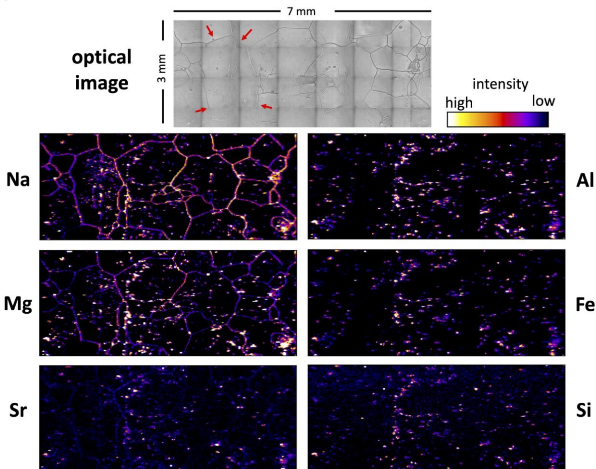
Figure 2. LA-ICP-MS elemental maps of Area 2 (3 x 7 mm) combined with a mosaic of optical images of the ice surface in the ablation chamber (top). Na and Mg show high intensities tracking the grain boundary network. All elements show dispersed bright spots at grain boundaries and in grain interiors. Red arrows in the optical image mark the same ice grain as in Figure 1 for reference.
