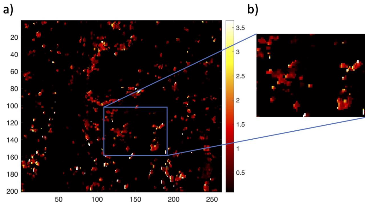
Figure 7. The Al/Na elemental mass ratio for locations determined by Al thresholding in Area 2 (see text). Panel a) shows the full map with a zoom-in to blue square shown in b). Note that the particle clusters generally show a large degree of heterogeneity in their elemental ratios, indicating a heterogeneous composition.
