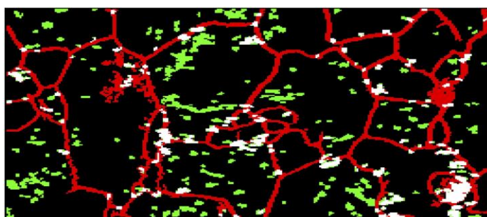
Figure 8. Example from Area 2 for a tentative differentiation of insoluble particle clusters located at grain boundaries (white) versus in the grain interior (green). Note that some misclassifications exist due to imperfect segmentation of the grain boundary network (see text).
