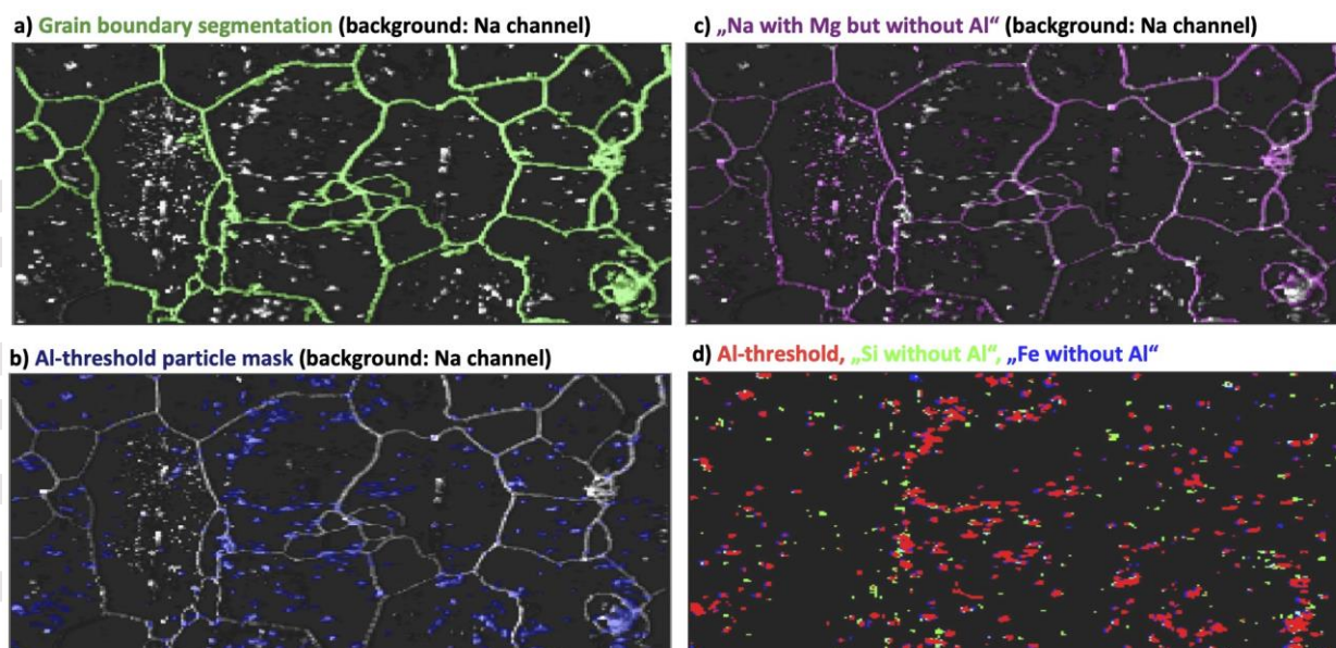
Figure 6. Illustration of the image segmentation and classification masks employed, using Area 2 as an example. Panel a) shows the grain boundary segmentation using a watershed algorithm (HDIP) in green, with the Na channel shown in white as background. Panel b) shows the particle mask obtained from thresholding of the Al channel (in blue, Na channel white in background). Panel c) shows the classification of “Na with Mg but without Al” (in pink, illustrated on top of the Na map, unselected pixels white in background). Panel d) shows the Al threshold in red together with “Si without Al” and “Fe without Al” in green and blue, respectively.
