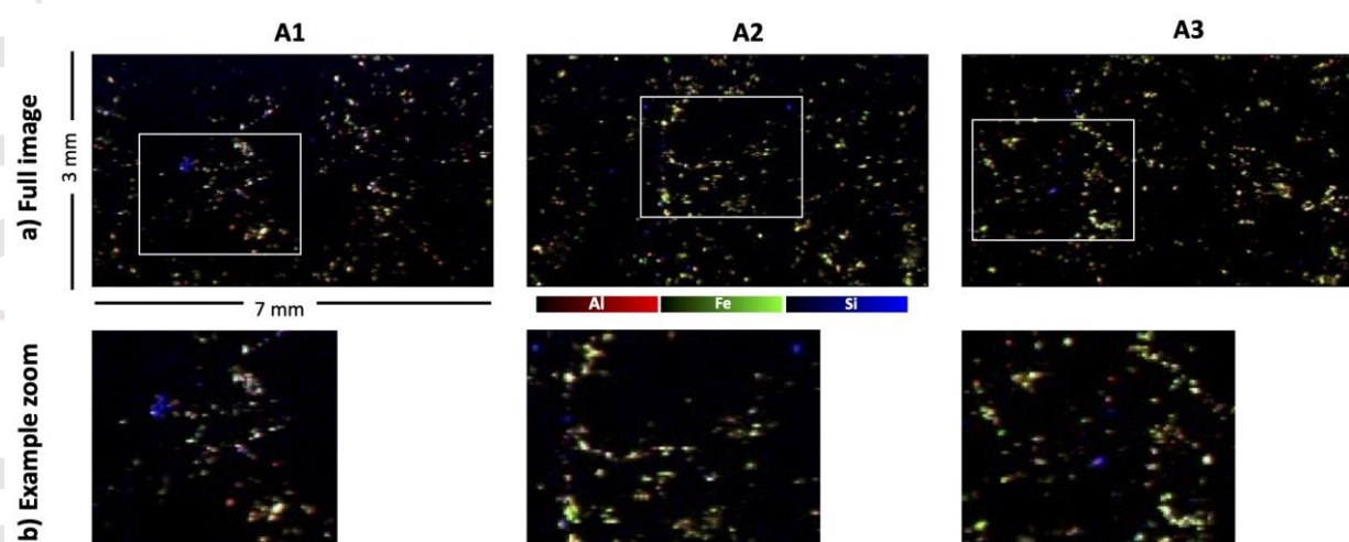
Figure 4. Visual colocalization analysis between Al, Fe and Si for the three areas, with their intensities shown in red, green and blue, respectively. Colocalization between Al and Fe are abundant (yellow) and also frequently found for all three elements (white). Occasionally, Si also occurs individually (blue spots). The top row shows the full elemental maps (a) and the bottom row (b) provides an example zoom-in for the areas marked by white rectangles in a).
