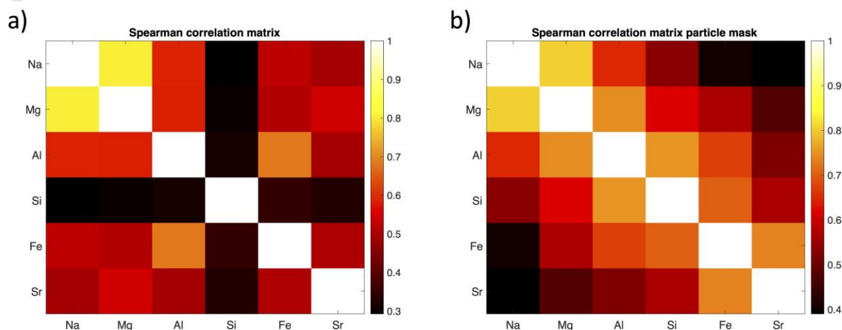
Figure 3. Correlation matrix showing the Spearman's correlation coefficient among all chemical elements for the logarithmic intensities obtained from the combined maps A1, A2 and A3 (a). Shown in b) are the correlations after segmentation of the bright spot image features via thresholding of the Al channel (see text).
