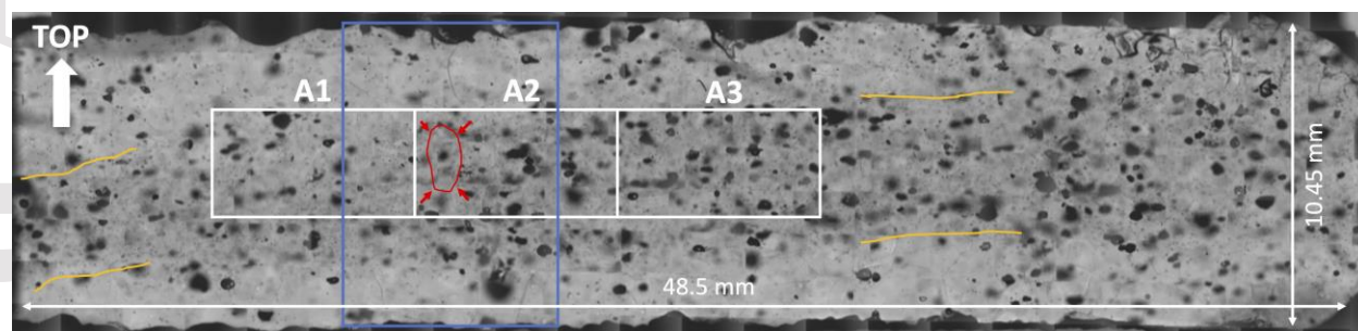
Figure 1. Microstructure mapping mosaic of optical images recorded prior to cryo-Raman analysis. The locations of the three areas analyzed by LA-ICP-MS at 20 \mu\text{m} resolution are indicated as white boxes (A1-A3). The location of the cryo-Raman analysis of S10 in Stoll et al. (2022) is shown as a blue box for reference. The cloudy band is visible as a slightly darker band running quasi-horizontally through the sample. For better visibility, approximate boundaries of the cloudy band are indicated by yellow lines. Red arrows point to an ice grain that stands out by its elongated vertical shape (outlines traced in red) and thus can be used as a reference to the elemental map A2. Note that this is a small slice of an ice core and the arrow “TOP” points towards the top of the core (i.e. the surface).
