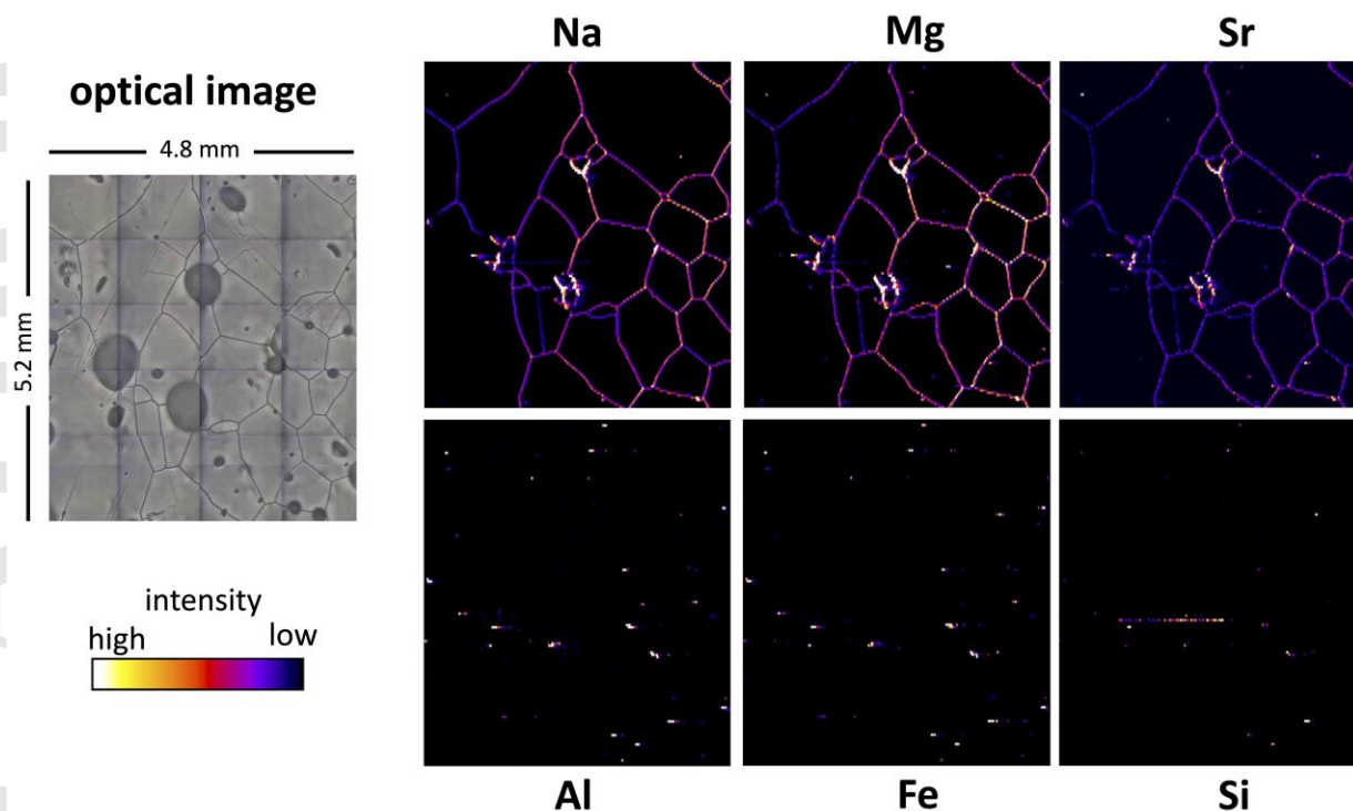
Figure 9. Comparison of the identical analytes as in the EGRIP sample, here obtained in a sample from MIS2 in the EPICA Dome C ice core. Albeit not as abundant, dispersed bright spots are also visible, especially within Al, Fe and to a limited extent also in Si. The bright horizontal line in the lower half of the Si map is an artifact.
