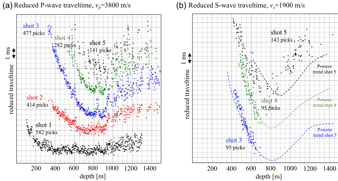
Figure 7. Traveltime measurements. (a) Reduced P -wave traveltime, t_0 - \sqrt{h^2 + \Delta^2}/v_p^0 , with a P -wave reduction speed of v_p^0 = 3800 \text{ m s}^{-1} . The actual origin time t_0 for the different shots is unknown. Specific values for t_0 are selected here merely for the purpose of producing a useful summary plot. (b) Reduced S -wave traveltimes, similar to panel (a), with an S -wave reduction speed of v_s^0 = 1900 \text{ m s}^{-1} . For comparison, the P -wave traveltime trends from panel (a) are superimposed in the form of dashed lines for shots 3, 4 and 5.
