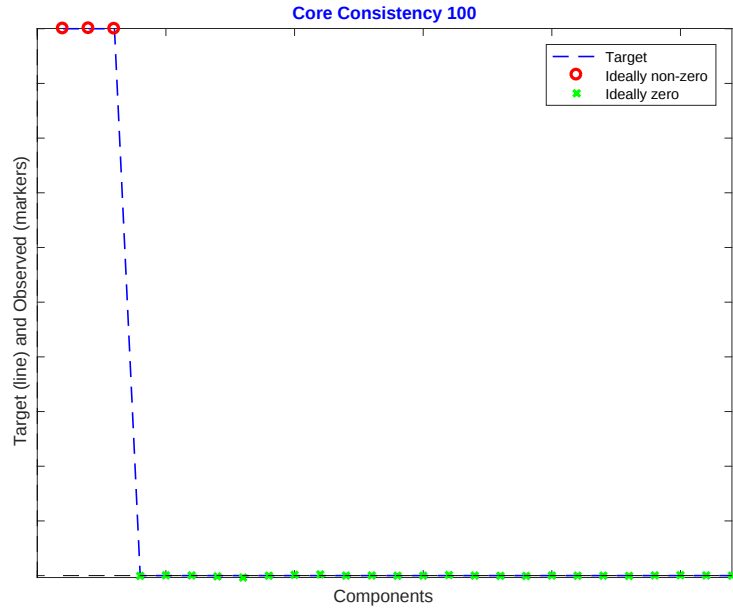
Figure 18: Corcondia 3 components.
