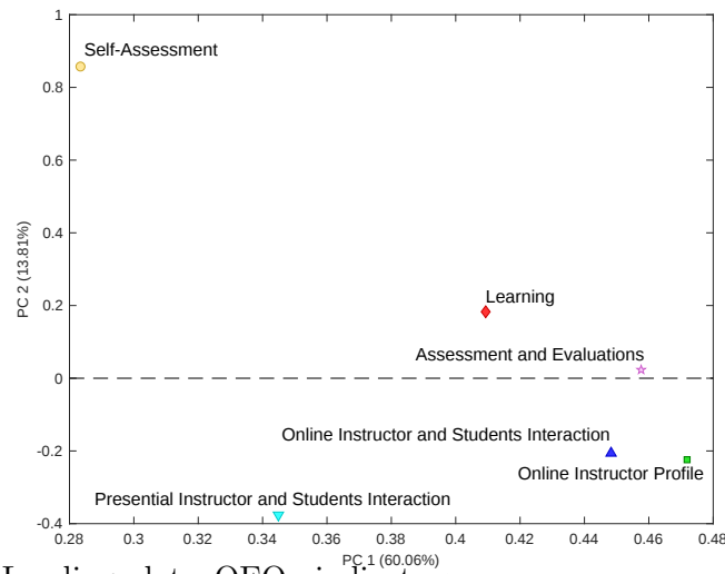
Figure 17: Loading plot - QEOn indicators.
